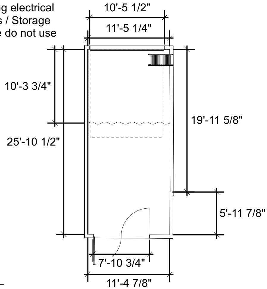
2 Top View with Dimensions Scale: 1/8" = 1'-0"
